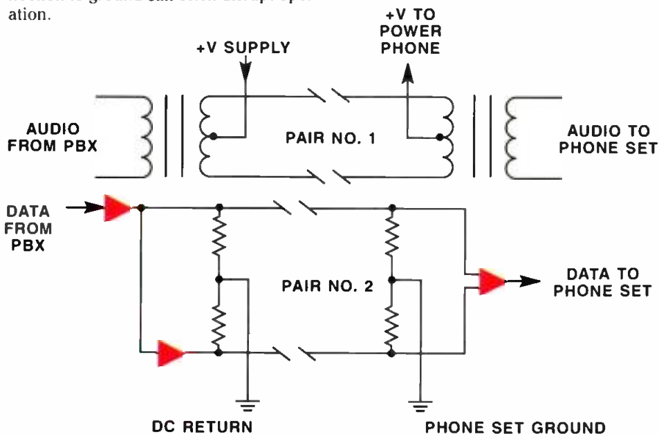
Figure 1. A common electronic phone wiring scheme using two pairs and phantom power. (Diagram shows data flow in only one direction for simplicity.)
