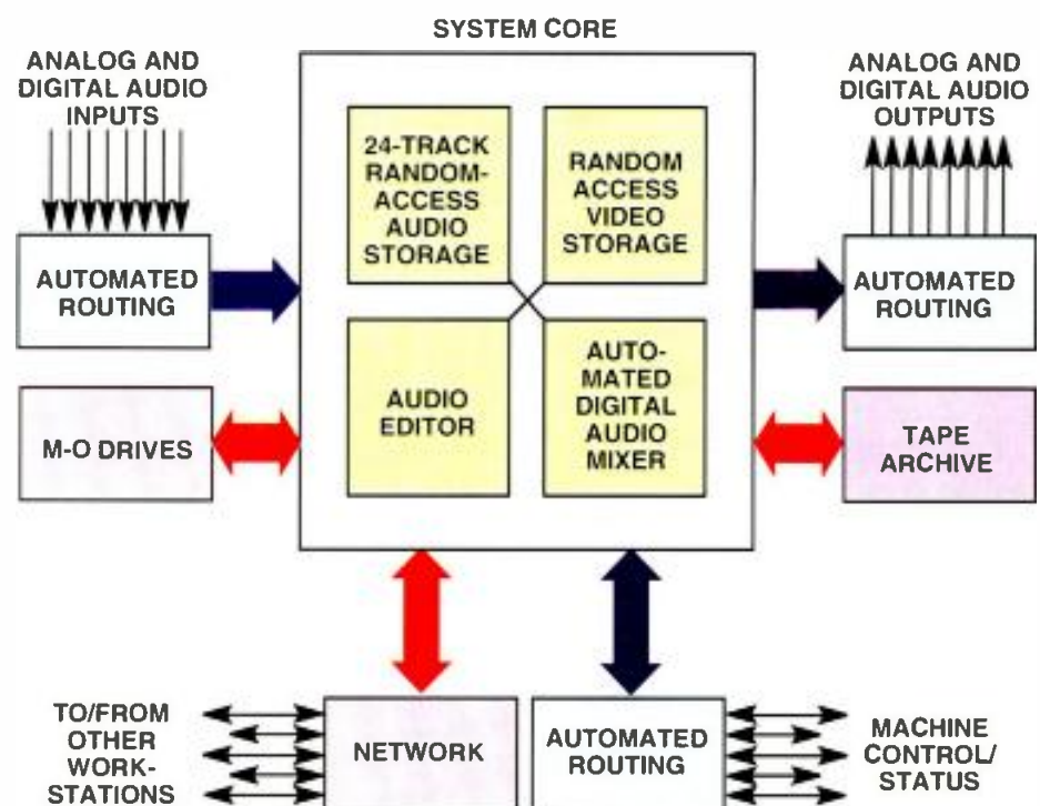
Figure 1. Conceptual block diagram of the Scenaria system.
